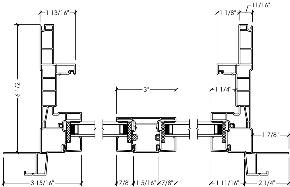
B PLAN DETAIL FIXED-FIXED
