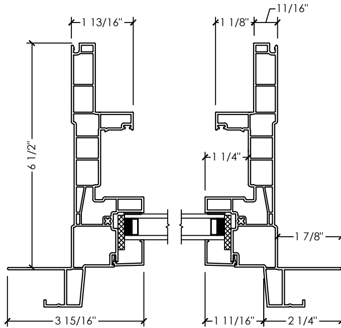
B PLAN DETAIL FIXED
