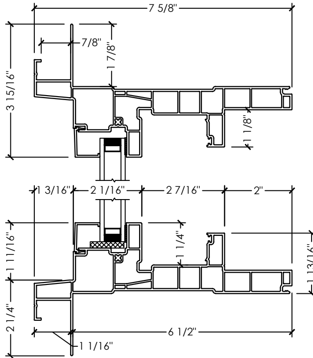
A SECTION DETAIL FIXED
