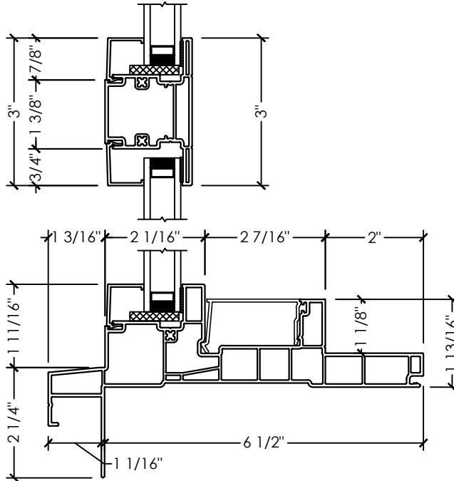
A SECTION DETAIL FIXED OVER FIXED
