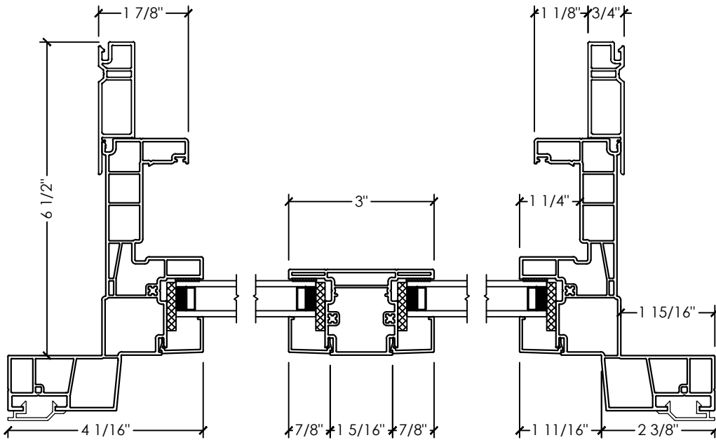
B PLAN DETAIL FIXED-FIXED
