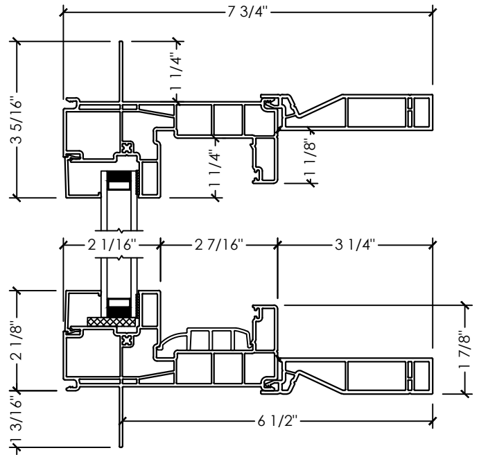
B SECTION DETAIL SINGLE SLIDER FIXED
