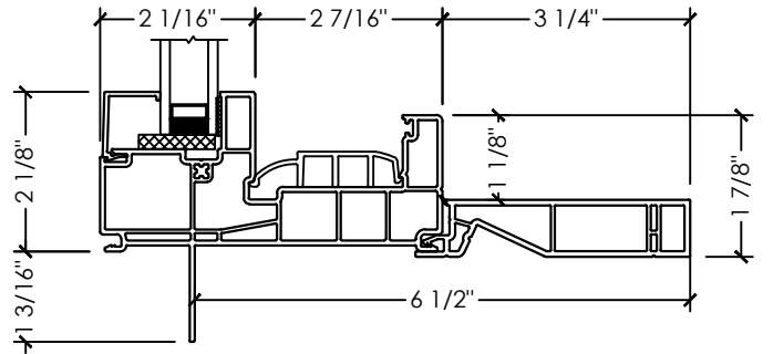
B SECTION DETAIL FIXED OVER FIXED
