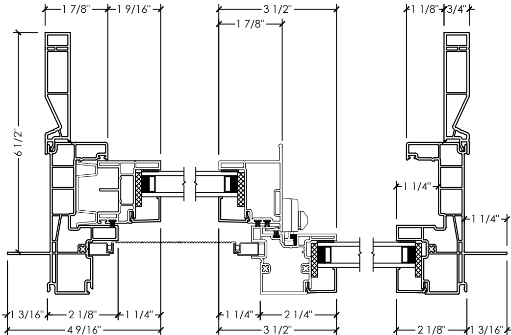
C PLAN DETAIL SINGLE SLIDER
