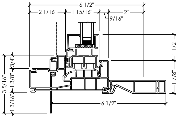
A SECTION DETAIL FIXED OVER SLIDER SASH
