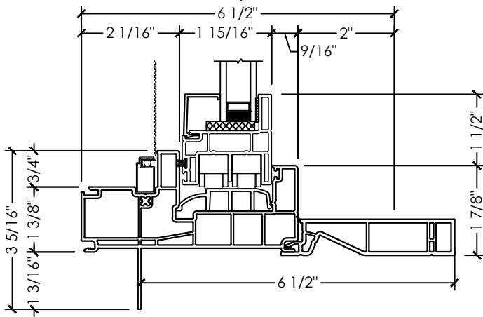
A SECTION DETAIL SINGLE SLIDER FIXED
