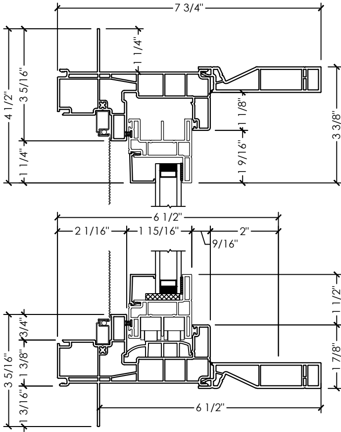
A SECTION DETAIL SINGLE SLIDER FIXED
