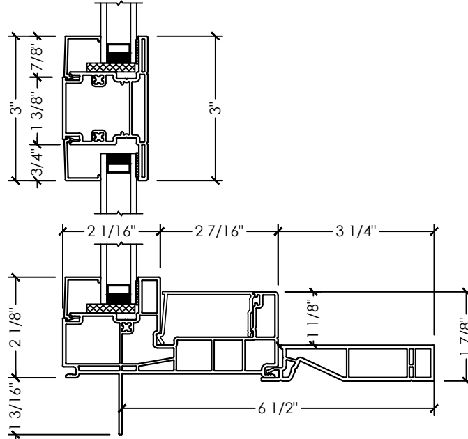
A SECTION DETAIL FIXED OVER FIXED
