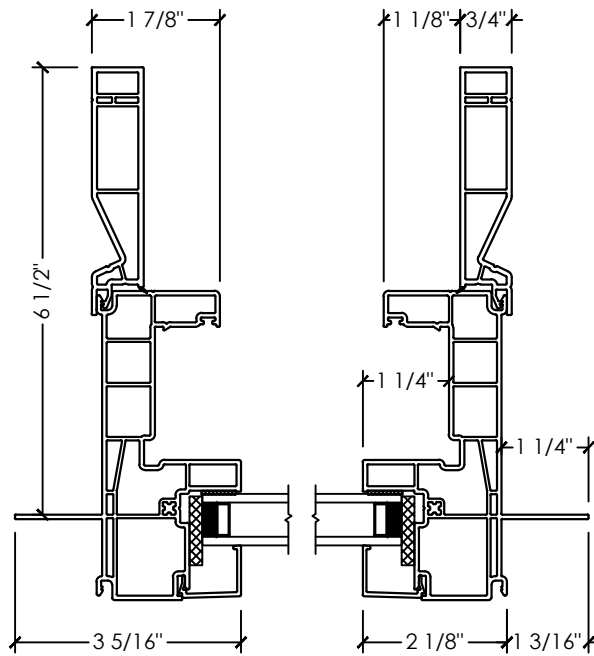
B PLAN DETAIL FIXED
