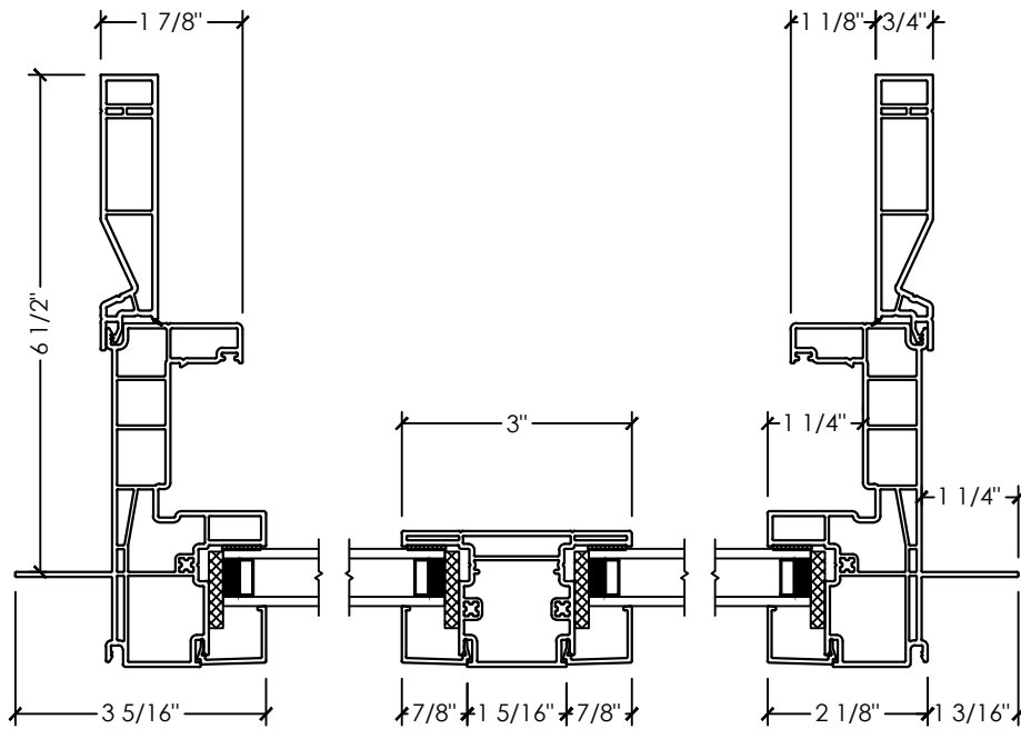
B PLAN DETAIL FIXED-FIXED
