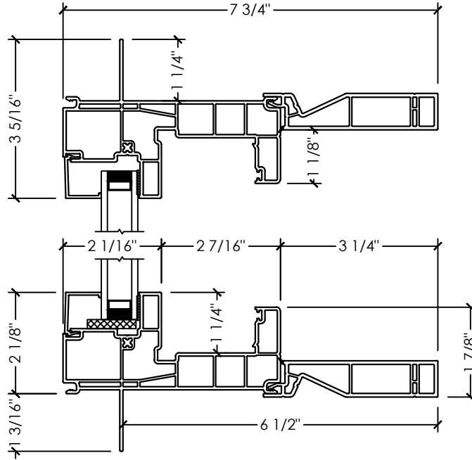
A SECTION DETAIL FIXED
