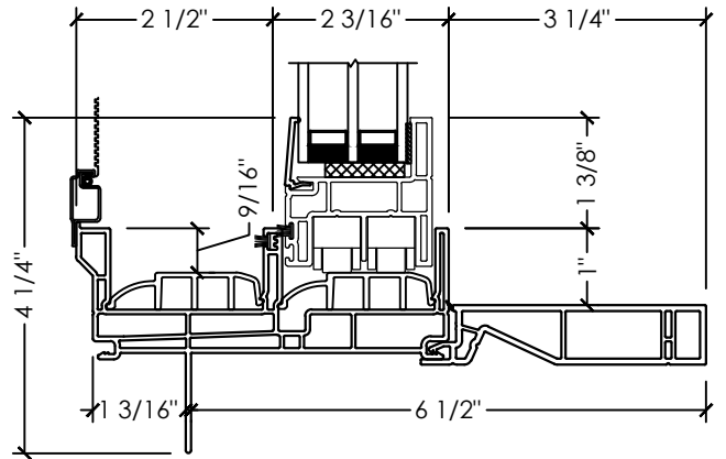
B SECTION DETAIL DOUBLE SLIDER - ACTIVE SASH
