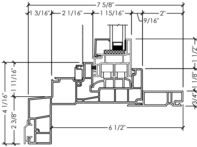
A SECTION DETAIL SINGLE SLIDER SASH
