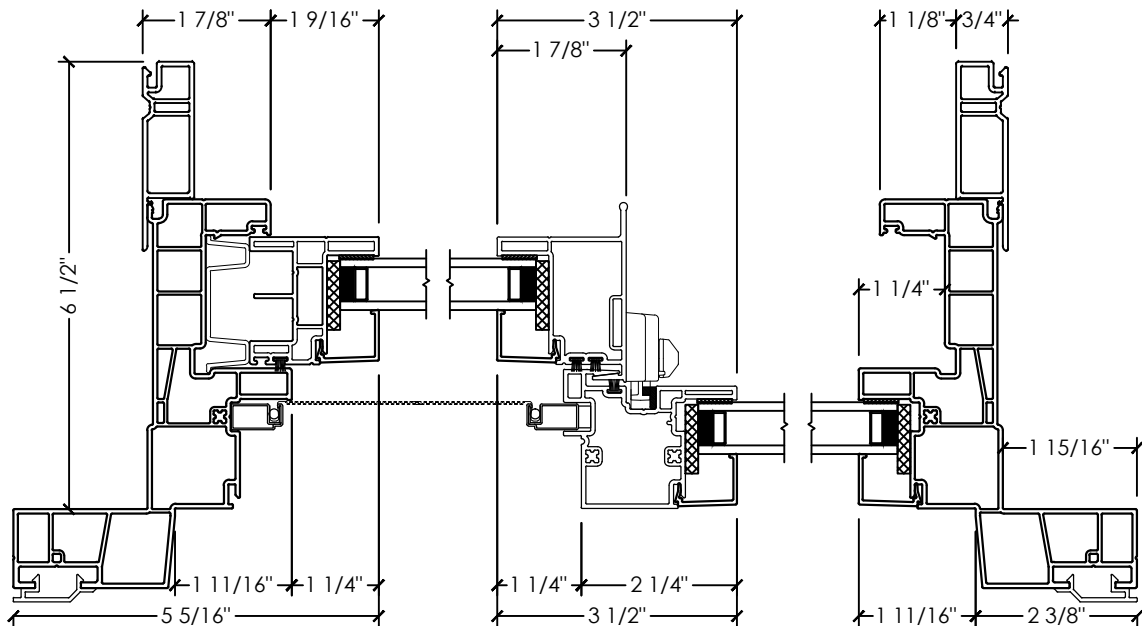
C PLAN DETAIL SINGLE SLIDER
