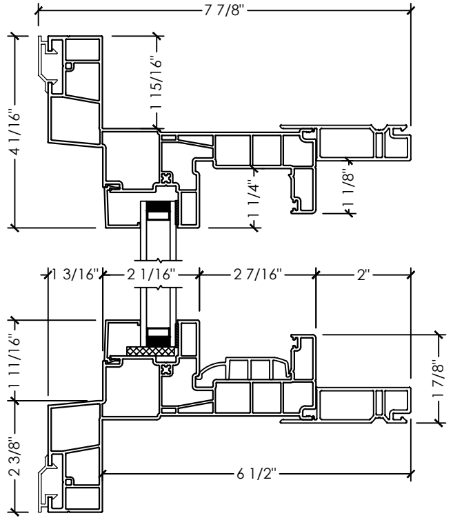
B SECTION DETAIL SINGLE SLIDER FIXED
