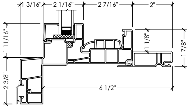
B SECTION DETAIL FIXED OVER FIXED
