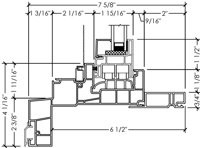
A SECTION DETAIL FIXED OVER SLIDER SASH
