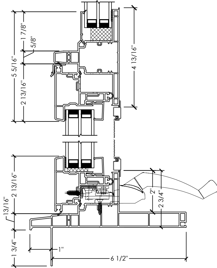
A SECTION DETAIL FIXED OVER AWNING
