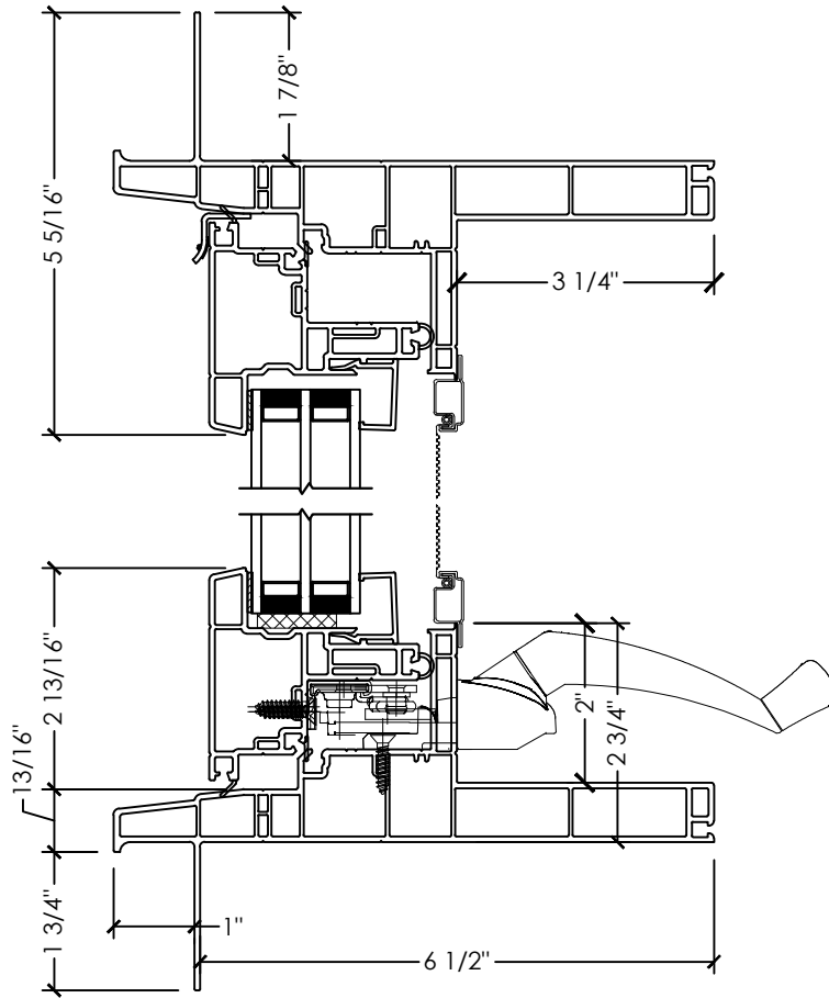
A SECTION DETAIL AWNING
