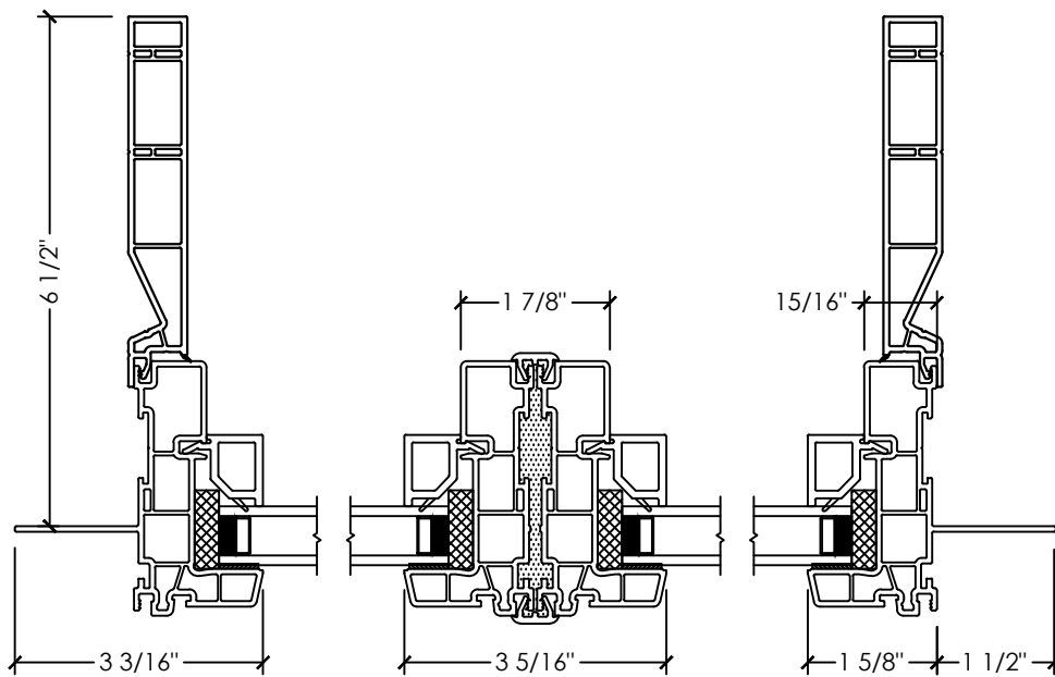
B PLAN DETAIL PICTURE-PICTURE
