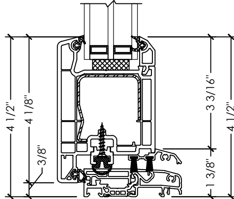
A SECTION DETAIL OUTSWING DOOR
