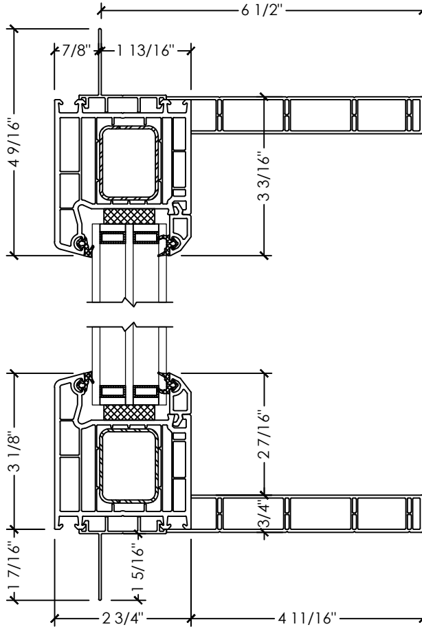
A SECTION DETAIL PICTURE (LARGE FRAME)
