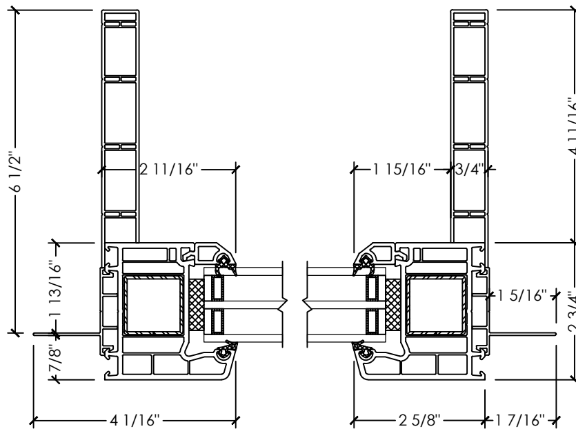
B PLAN DETAIL PICTURE (SMALL FRAME)
