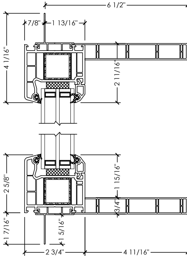
A SECTION DETAIL PICTURE (SMALL FRAME)
