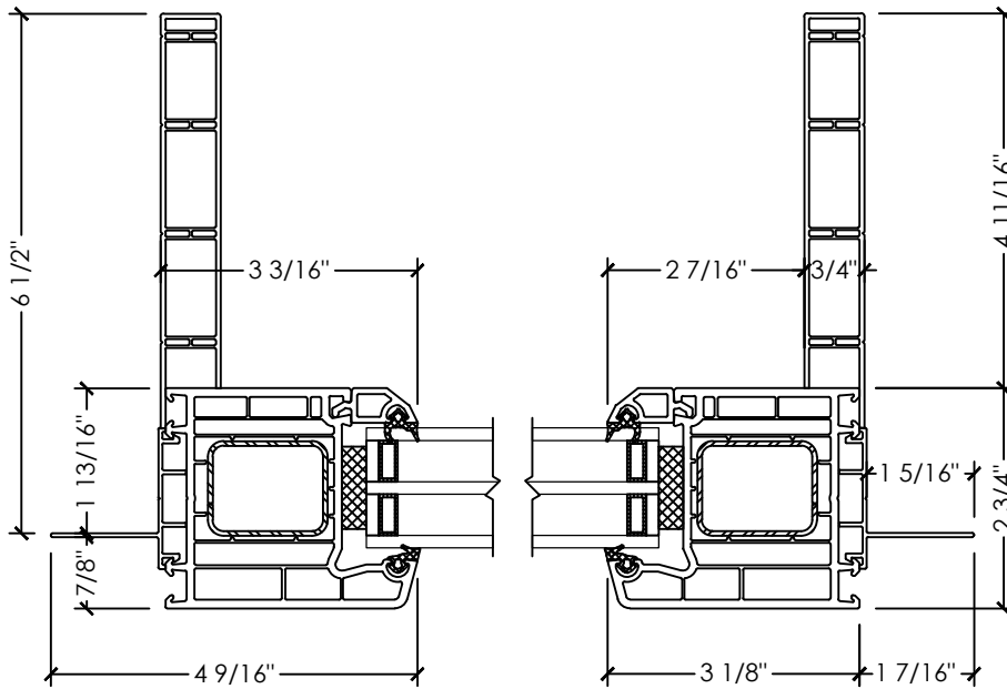
B PLAN DETAIL PICTURE (LARGE FRAME)
