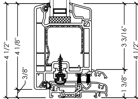
A SECTION DETAIL OUTSWING DOOR
