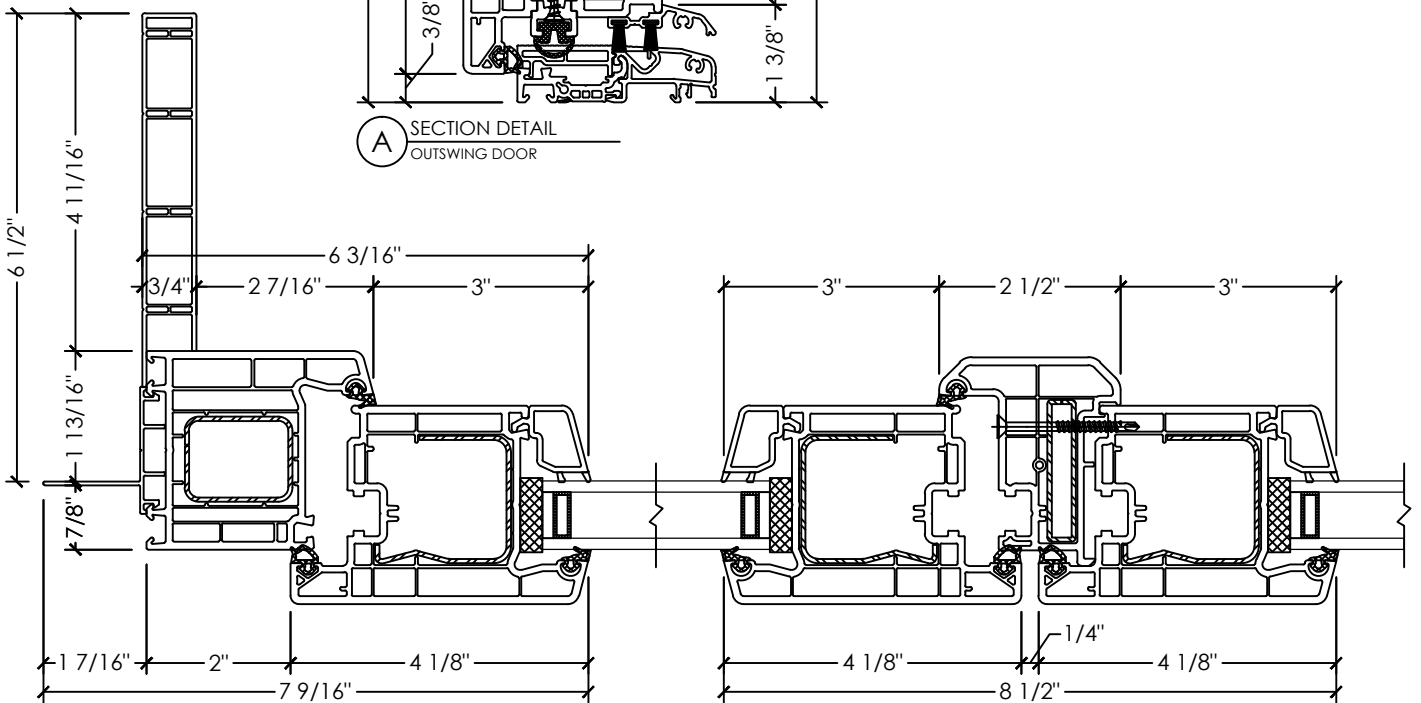
B PLAN DETAIL OUTSWING DOOR
