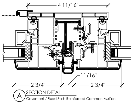
Casement / Fixed sash
