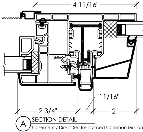
Casement / Direct Set
