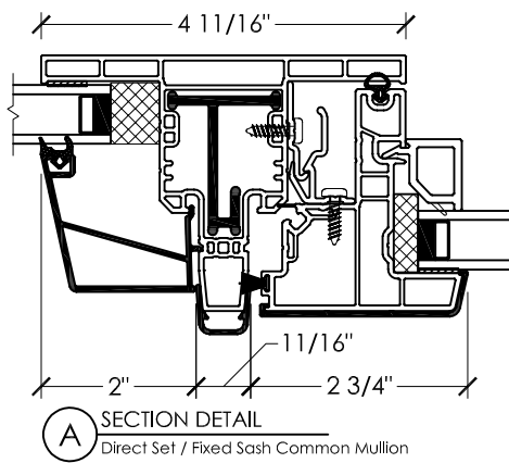
Direct Set / Fixed sash
