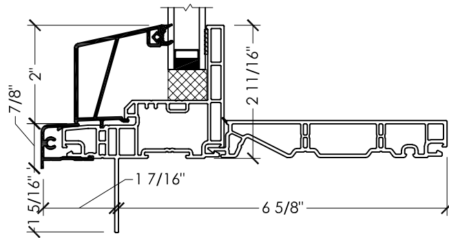
B SECTION DETAIL Head and Sill
