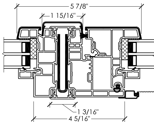
A SECTION DETAIL Picture / Casement Box-to-Box Mullion - 1/2" Reinforcement
