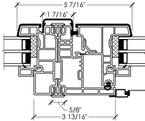
A SECTION DETAIL Picture / Casement Box-to-Box Mullion
