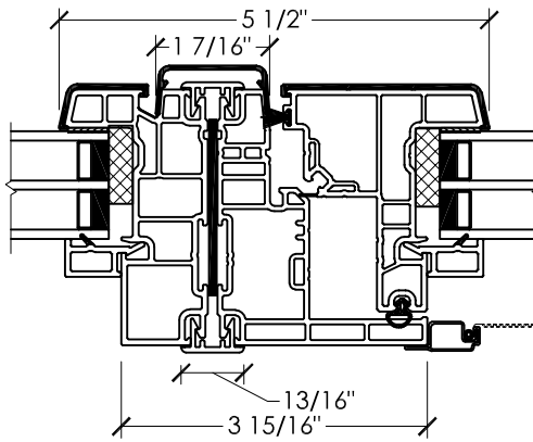
A SECTION DETAIL Picture / Casement Box-to-Box Mullion - 1/8" Reinforcement
