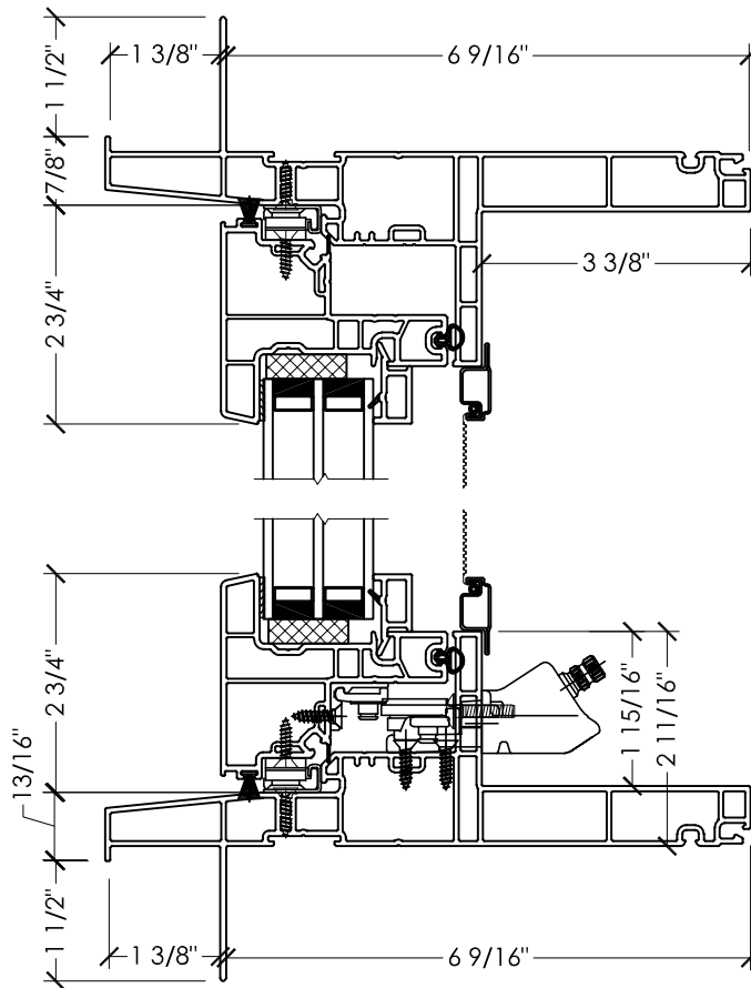
B SECTION DETAIL Head and Sill
