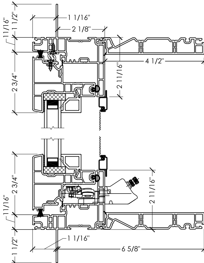
B SECTION DETAIL Head and Sill
