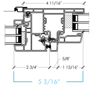
Common Mullion Casement / Fixed Sash
