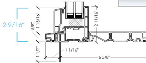
Continuous Frame Direct Set
