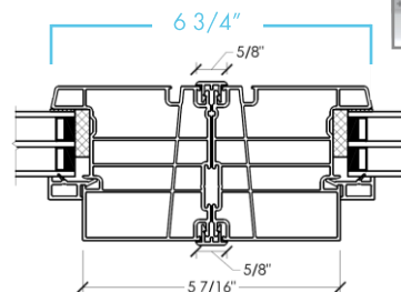
Box-to-Box Mull Fixed / Fixed
