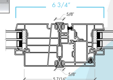
Box-to-Box Mull Fixed / Casement
