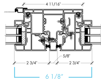
Box-to-Box Mull Picture / Casement
