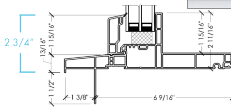
Monoframe Direct Set
