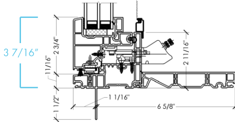
Continuous Frame Casement
