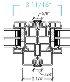
Box-to-Box Mull Fixed / Fixed
