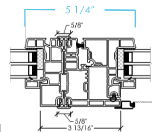
Box-to-Box Mull Fixed / Casement
